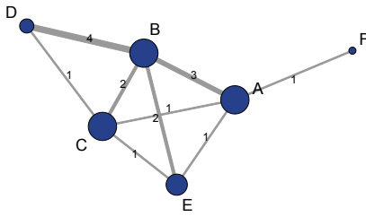
Figure 5: Example network.
