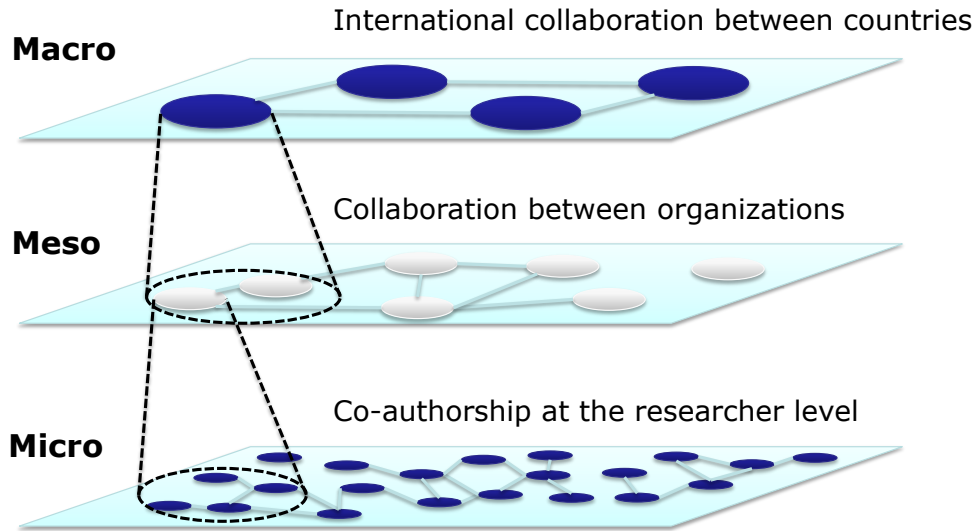
Figure 1: Multimodal structures
